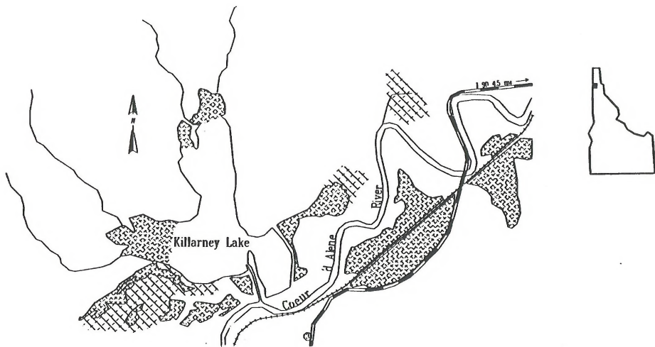
Figure 1. Map of Killarney Lake, one of the lateral lakes on the Coeur d' Alene River, near Harrison, Idaho.
